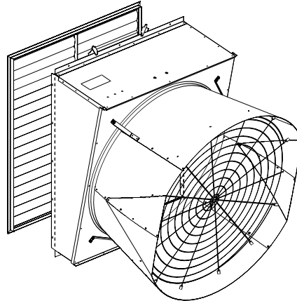
WF54 with C or CX style cone
